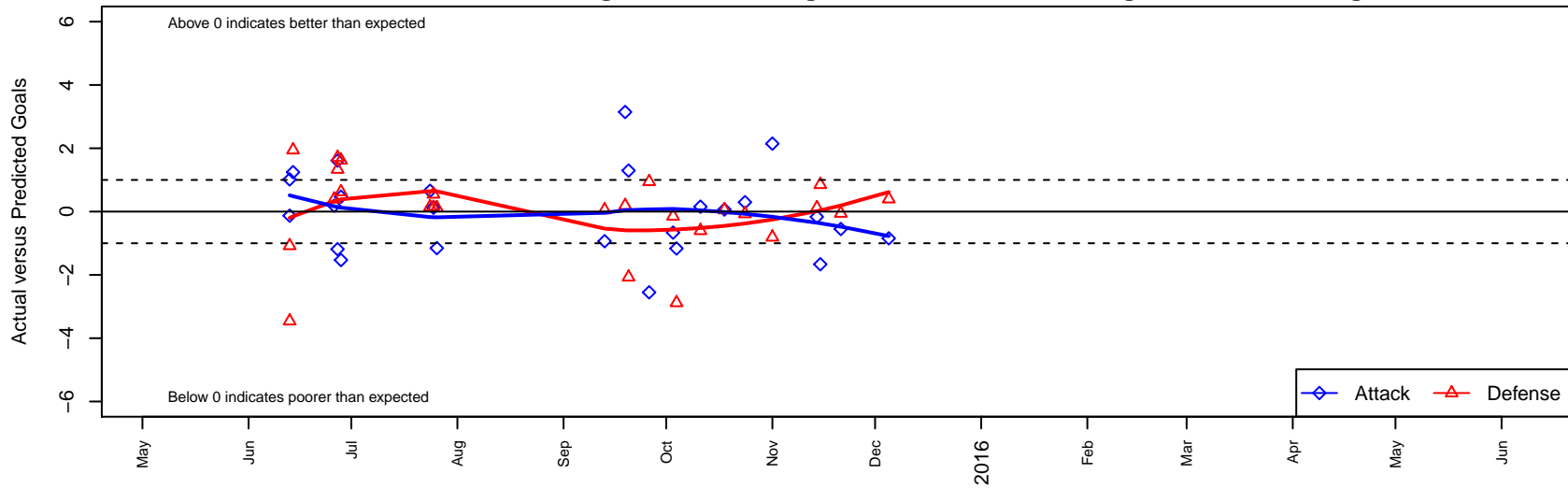
Gala FC 2000B Dots are actual minus expected GF (blue circles) and GA (red triangles). Blue line is smoothed change in attack strength. Red is smoothed change in defense strength.
